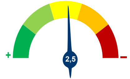
Scope ESG-Rating
